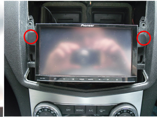
Ensure all wires are clear of the aperture. Slide the head unit back into the dash. Ensure that the guide knobs are lined up with the guide rails as shown.
